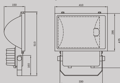
HQI-400
